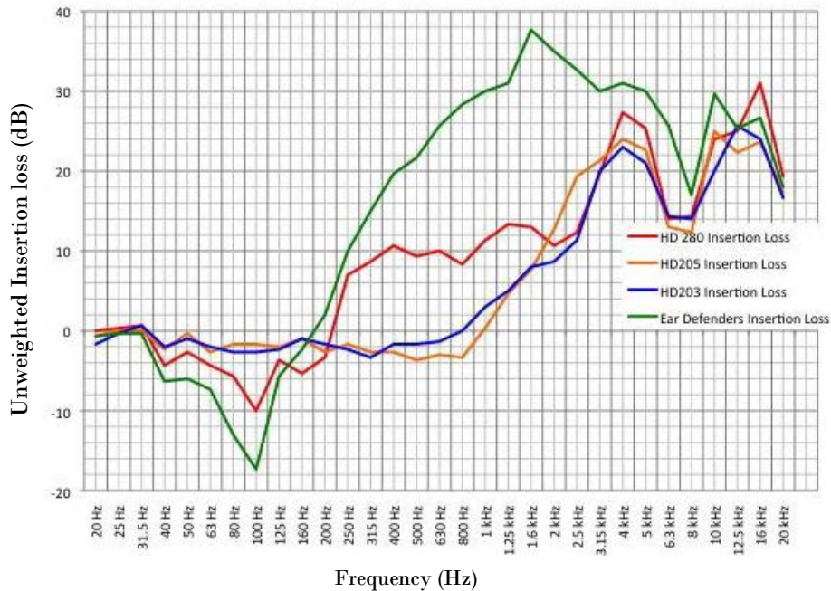
Figure 3 – Measured Insertion loss in dB of headphones and ear defenders across the audio spectrum (20Hz to 20 kHz)
