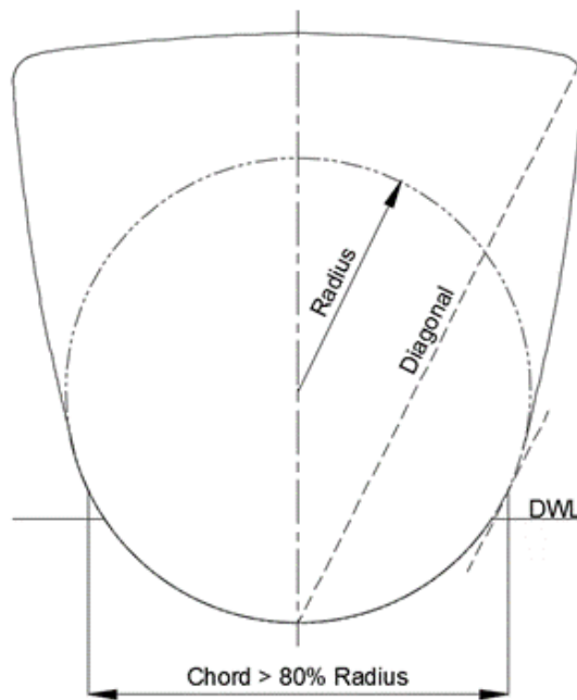
Figure 2: Natural stiffener criterion for circular center panel.
