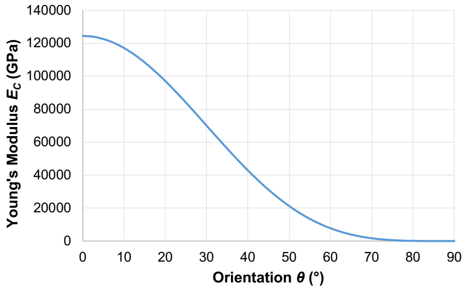
Figure 5: Variation in Young's modulus of a prepreg carbon UD with misalignment.
