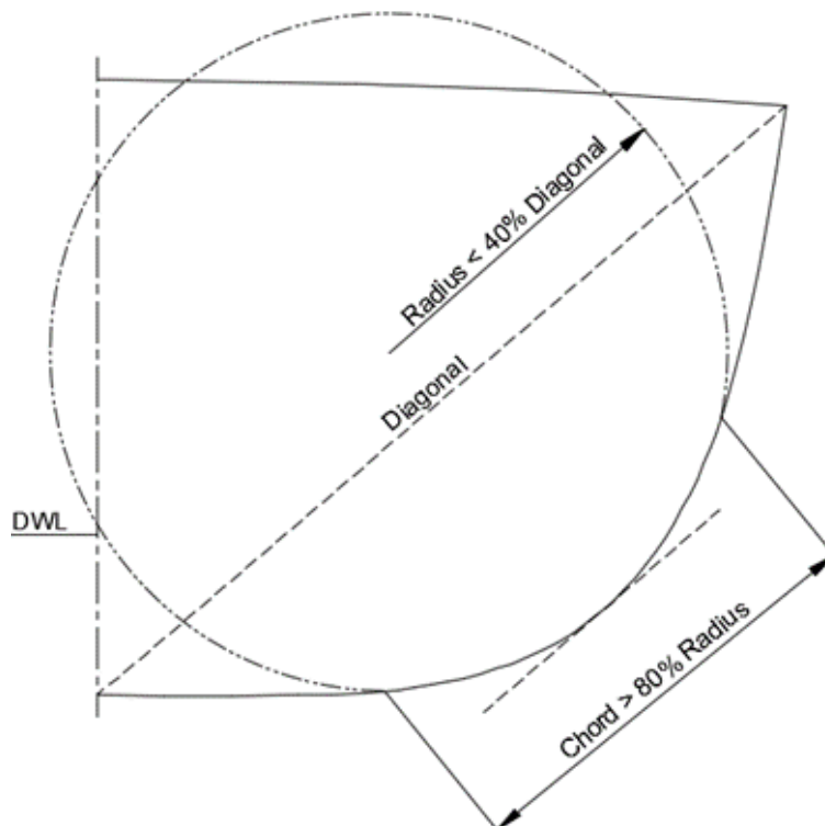
Figure 3: Natural stiffener criterion for curved panel.
