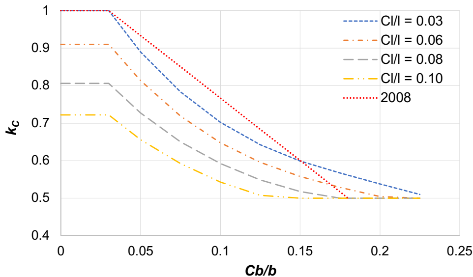
Figure 4: Curvature correction coefficients.
